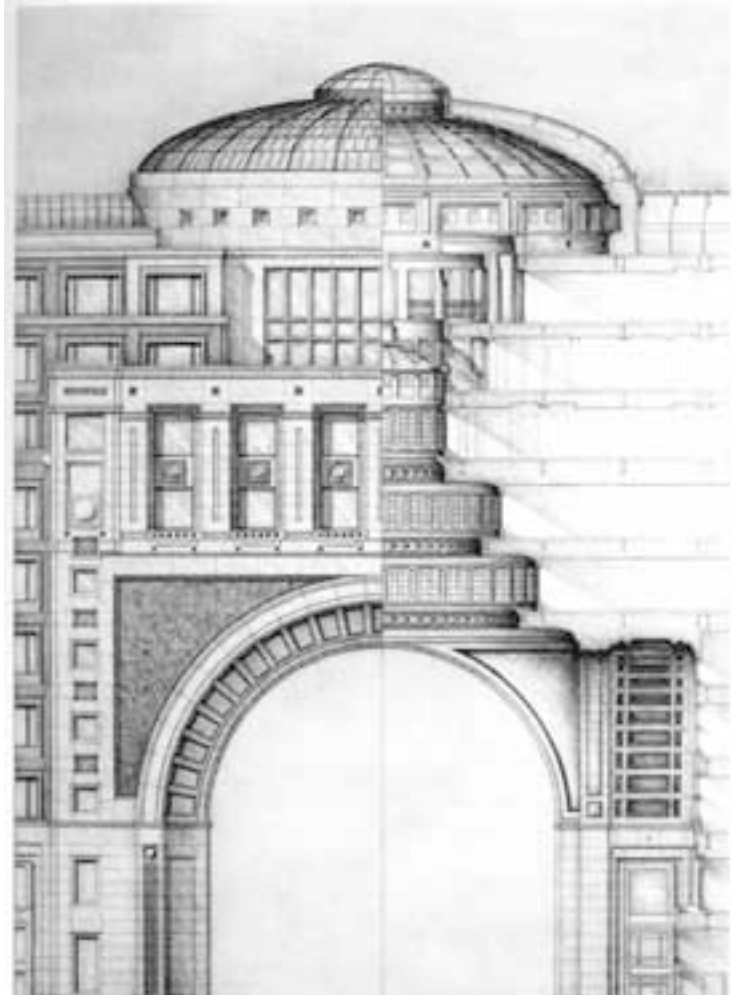
Rowers Wharf w Bostonie, Adrian Smith. 1982-87
